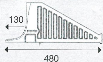
Anti trip foot
