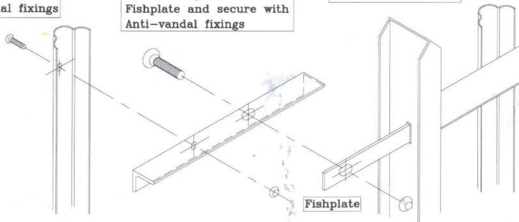
GENERAL FIXING ARRANGEMENT
