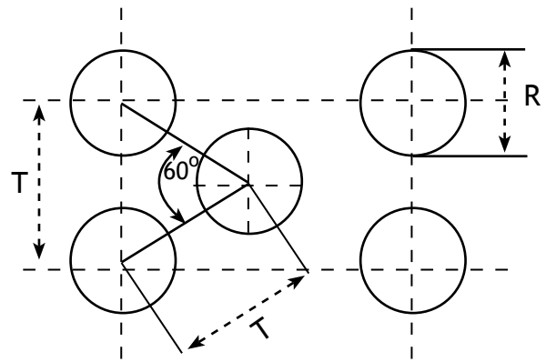
ROUND HOLES STAGGERED 60° PITCH
